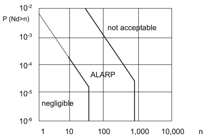
Figure 1 F - n -curves, where F(n) = P(N_d > n) in one year), and the ALARP region
