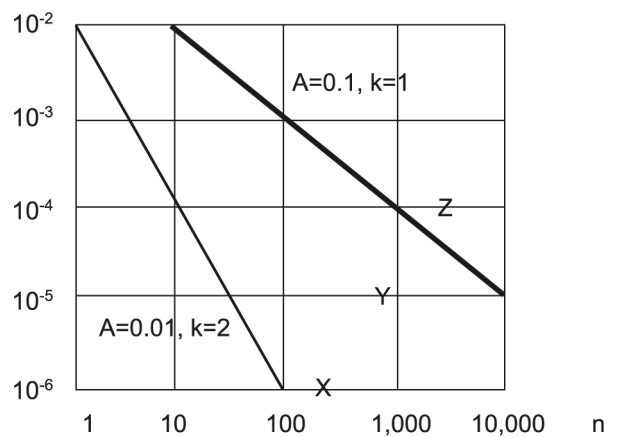
Figure 2 The F(n) = P(N_d > n) < A n^{-k} requirement for one year (see ISO 2394)
